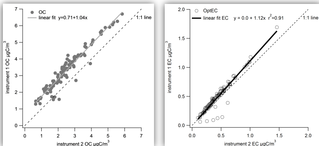
Figure 7. Collocated 24-hour OC (left) and OptEC (right) measurements at St. Louis during August 11, 2016, through January 11, 2017.
