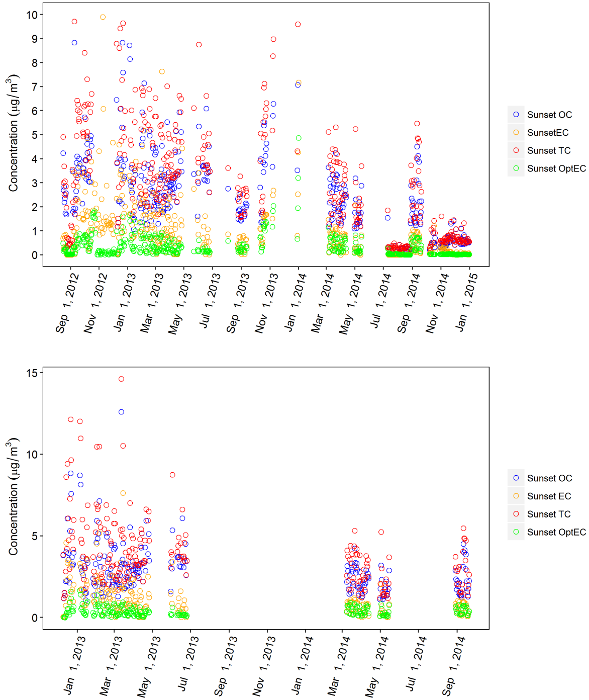
Figure B-3. Time series of Sunset data available in AQS (top) and data used in this work (bottom) for Las Vegas. Data were intermittent due to multiple operational issues. Only data with multiple weeks of consistent measurements were included for analysis. For example, in November 2012, OC was consistently reported as less than 0.5 \mu\text{g}/\text{m}^3 , and at other times the NDIR and heater coils broke multiple times, there was vandalism that incapacitated the shelter air conditioning unit, and instrument software was not routinely updated.
