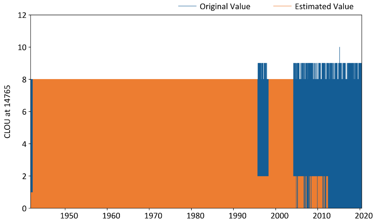
Figure A-24. The filled cloud cover data at gage 72506814765.
