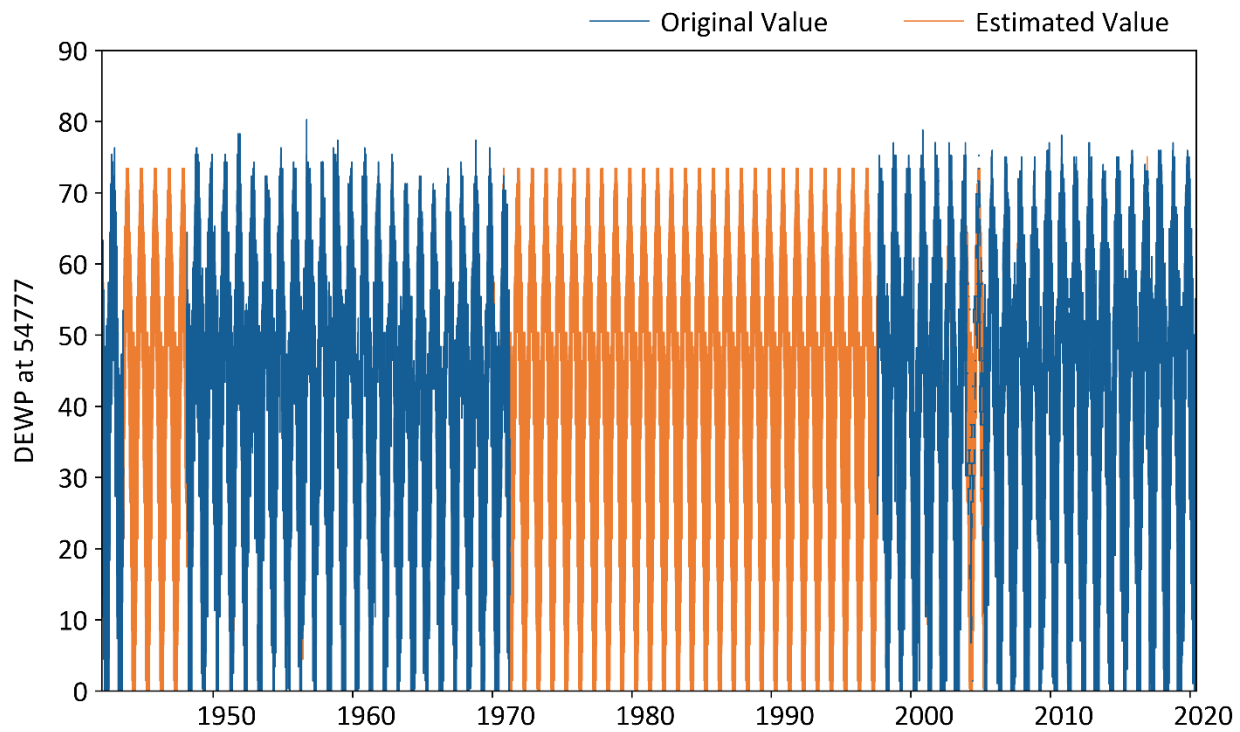
Figure A-20. The filled dew point temperature data at gage 72506854777.
