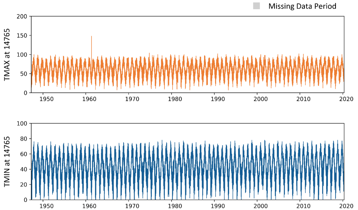
Figure A-6. The original daily temperature data at gage 72506814765.
