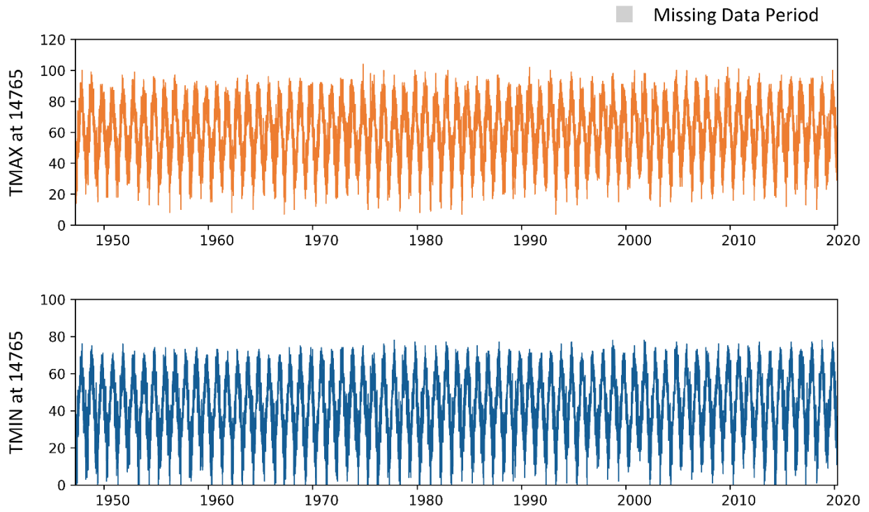
Figure A-9. The revised daily temperature data at gage 72506814765.
