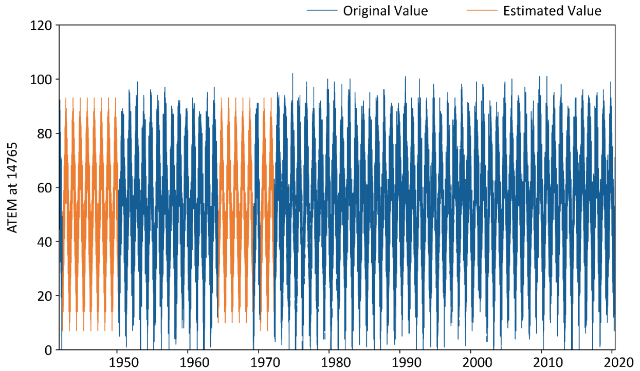
Figure A-14. The filled hourly temperature data at gage 72506814765.
