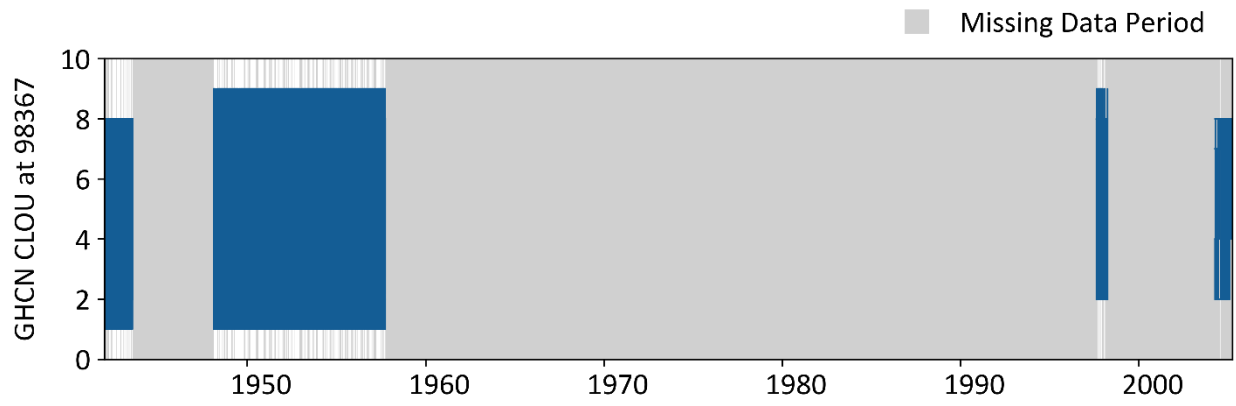
Figure A-23. The cloud cover data at gage 72506899999.
