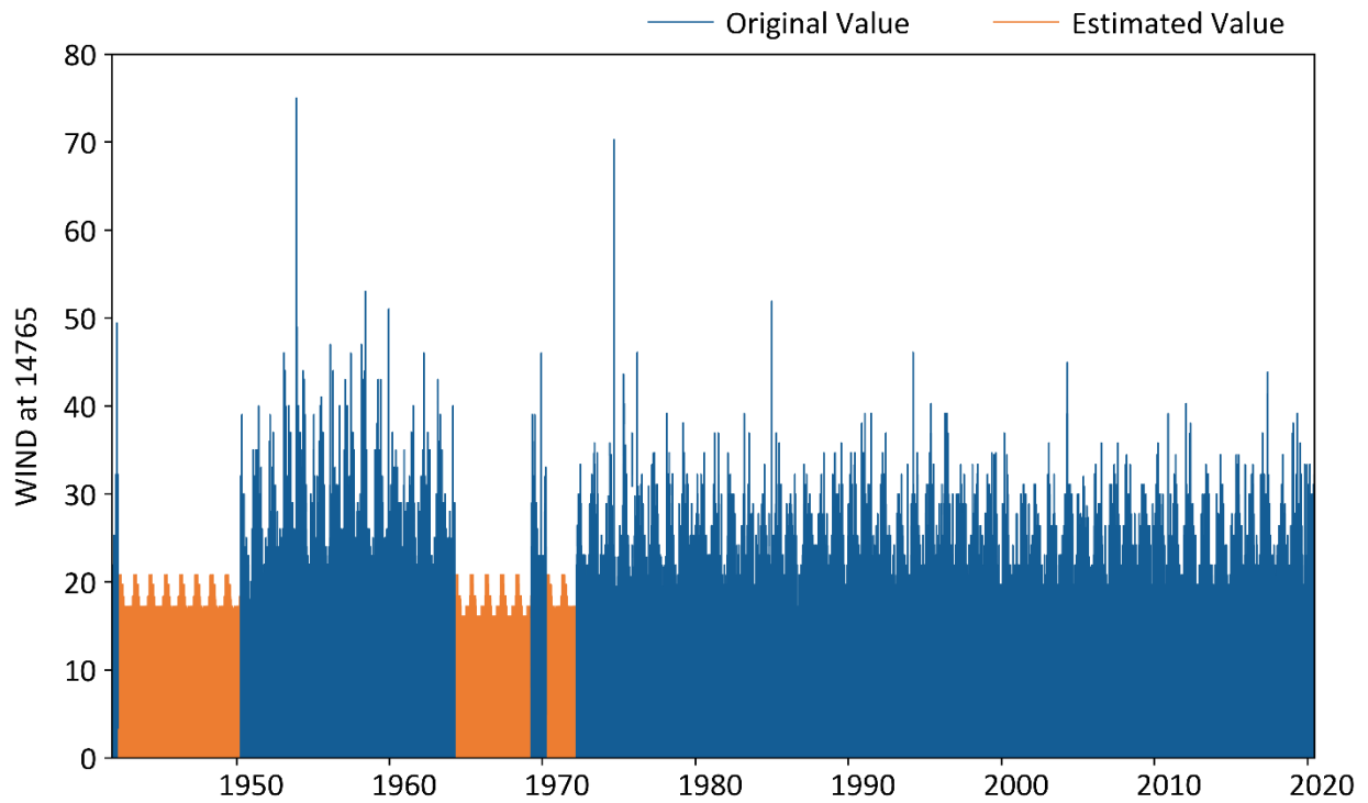
Figure A-4. The filled wind speed data at gage 72506814765.
