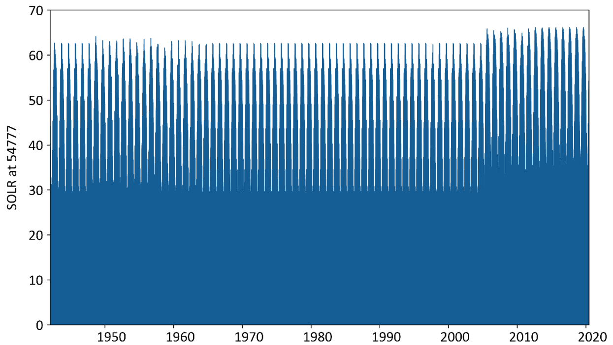
Figure A-27. The computed solar radiation data at gage 72506854777 using WDM Utility.
