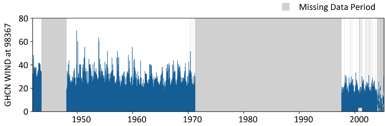
Figure A-3. The wind speed data at gage 72506899999.
