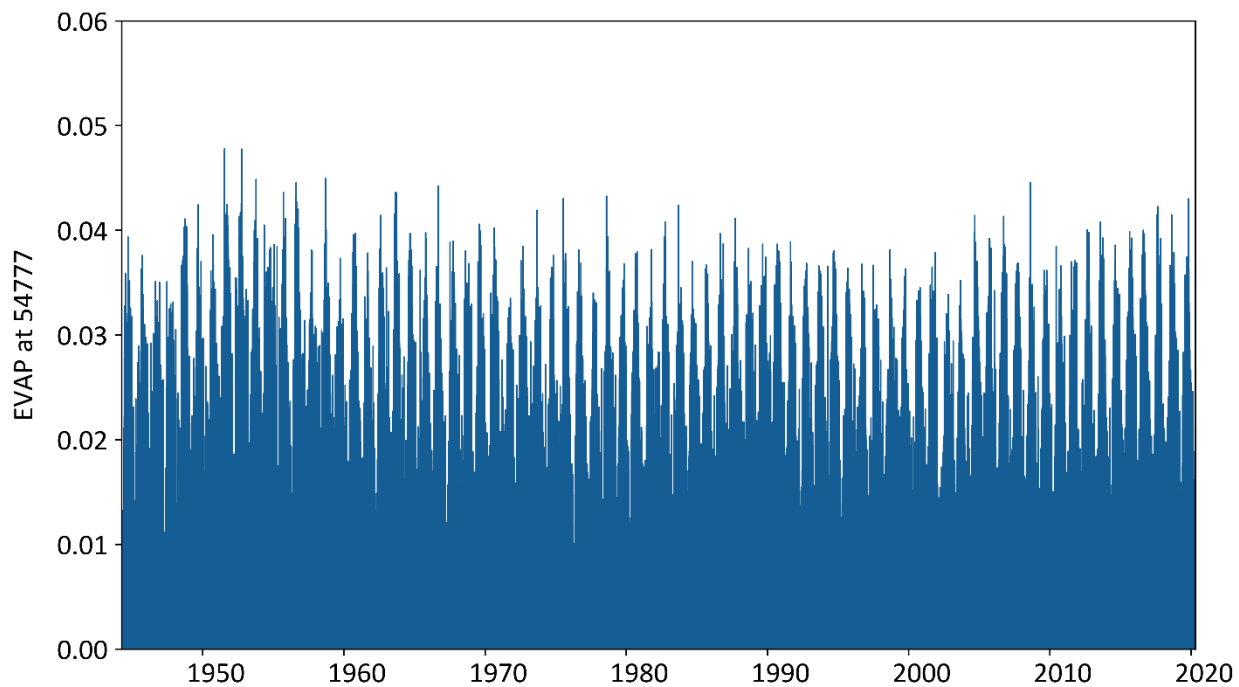
Figure A-29. The computed potential evapotranspiration data at gage 72506854777 using WDM Utility.
