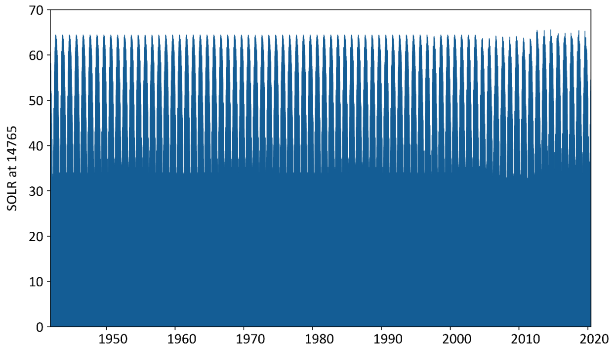
Figure A-26. The computed solar radiation data at gage 72506814765 using WDM Utility.
