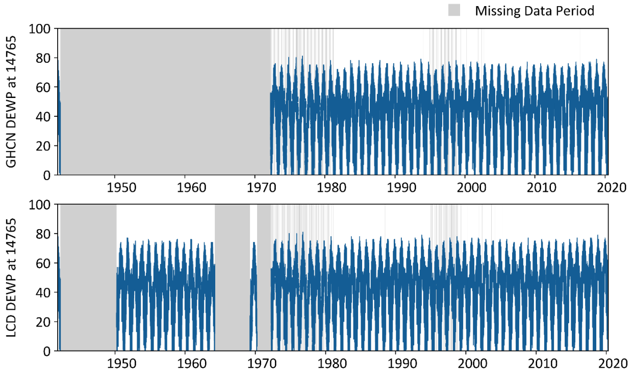
Figure A-16. The dew point temperature data at gage 72506814765.
