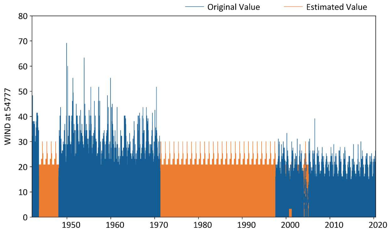
Figure A-5. The filled wind speed data at gage 72506854777.
