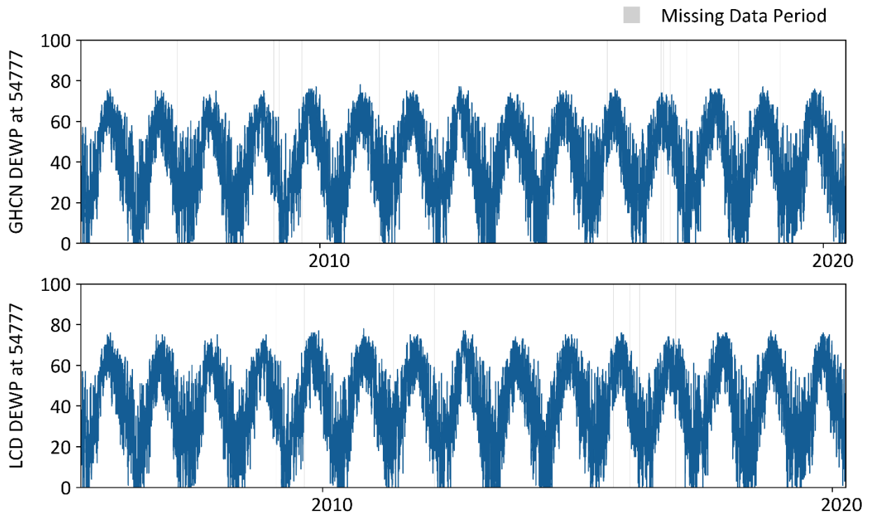
Figure A-17. The dew point temperature data at gage 72506854777.
