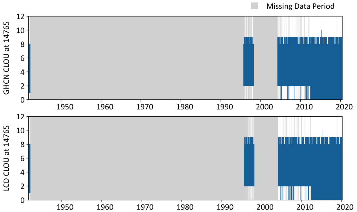
Figure A-21. The cloud cover data at gage 72506814765.
