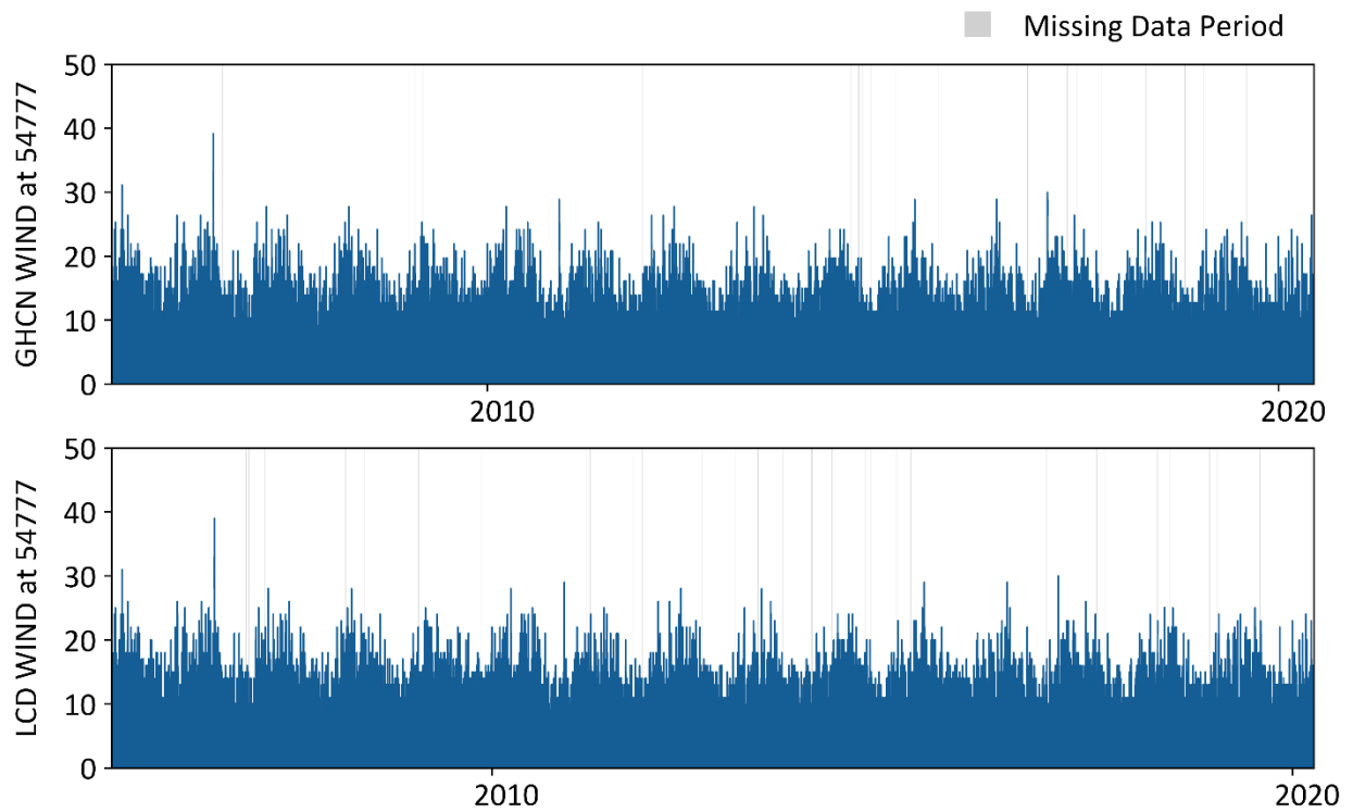
Figure A-2. The wind speed data at gage 72506854777.
