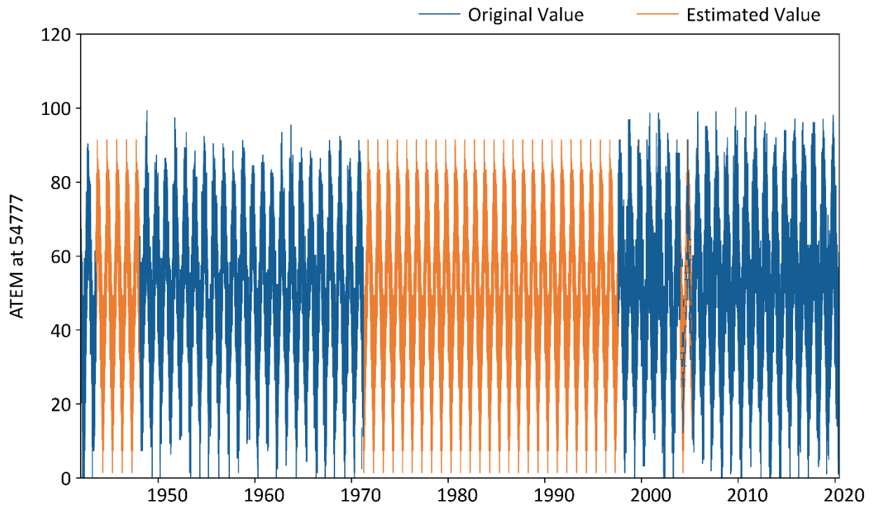
Figure A-15. The filled hourly temperature data at gage 72506854777.
