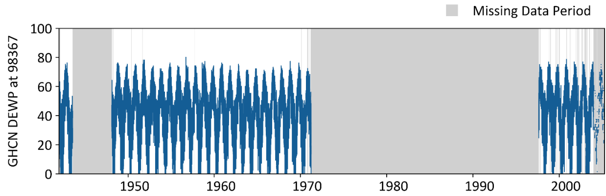
Figure A-18. The dew point temperature data at gage 72506899999.
