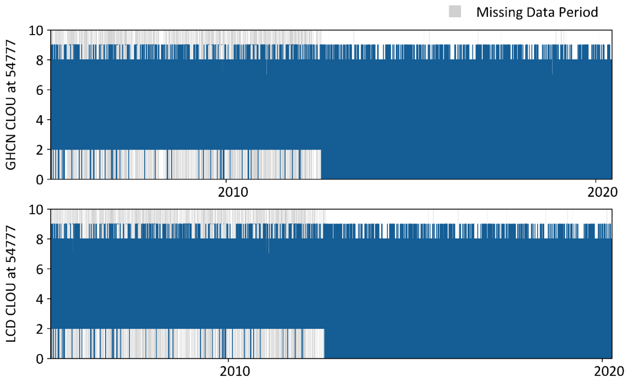
Figure A-22. The cloud cover data at gage 72506854777.
