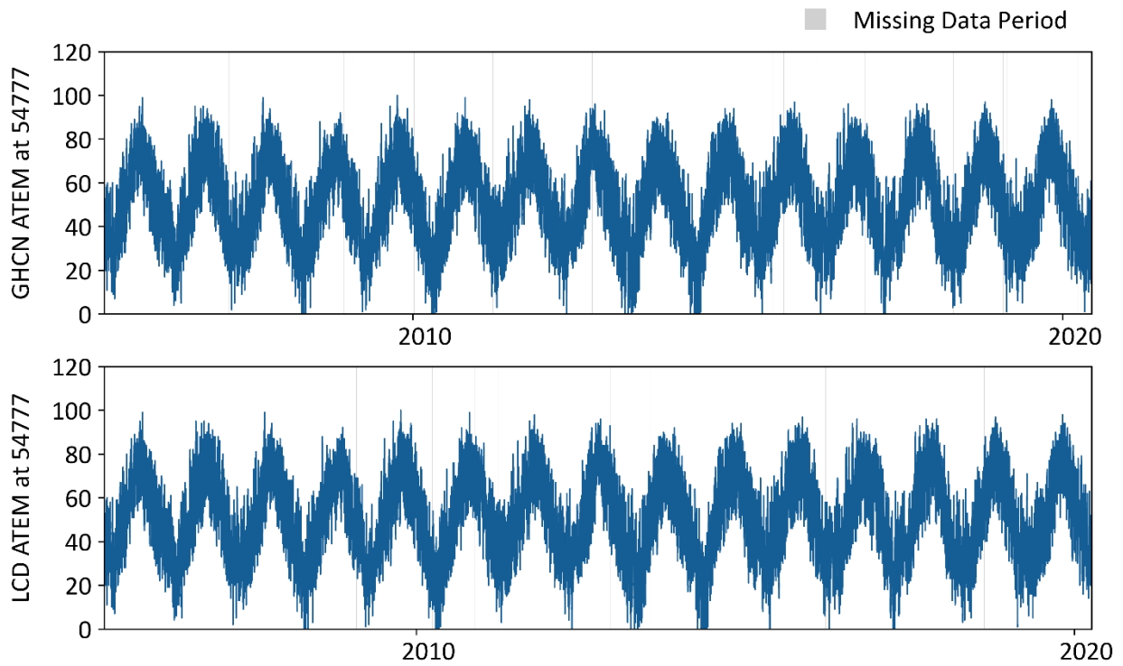
Figure A-12. The hourly temperature data at gage 72506854777.
