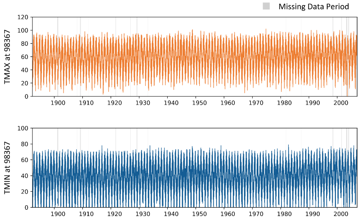
Figure A-8. The original daily temperature data at gage 72506899999.
