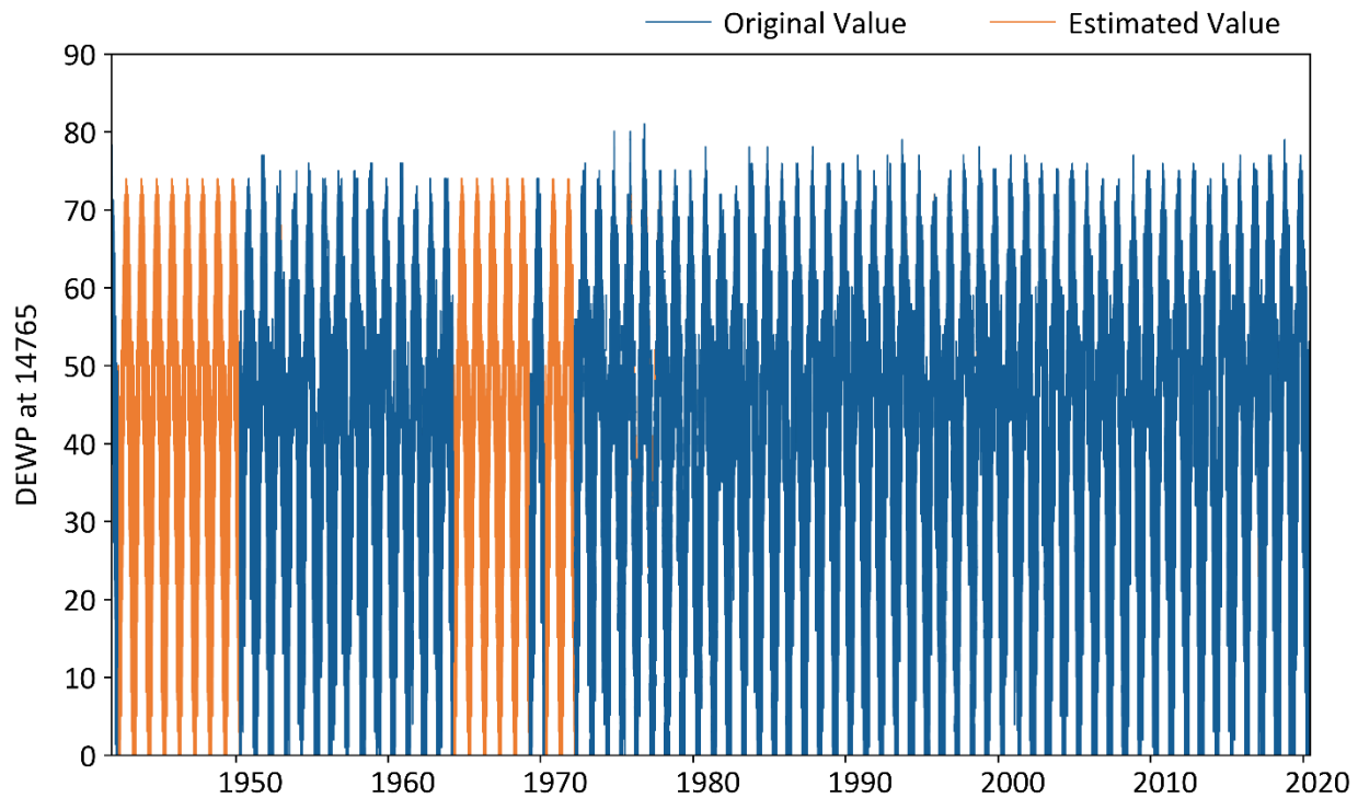
Figure A-19. The filled dew point temperature data at gage 72506814765.
