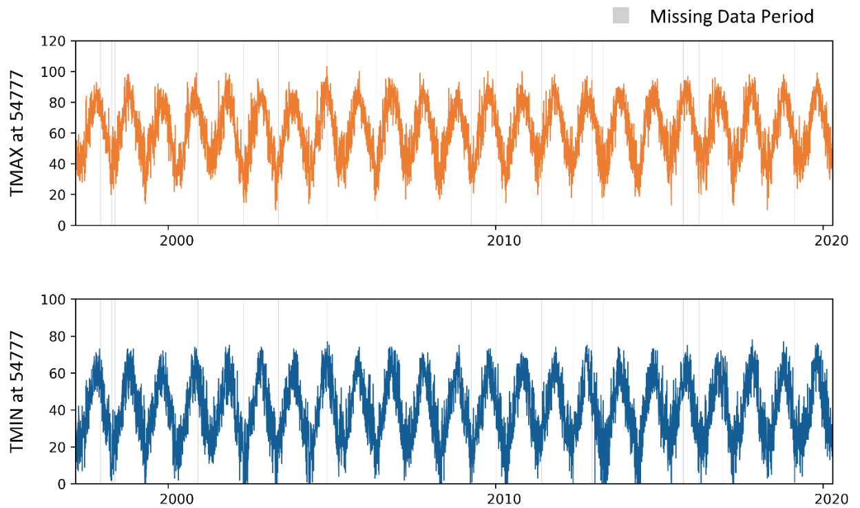
Figure A-7. The original daily temperature data at gage 72506854777.
