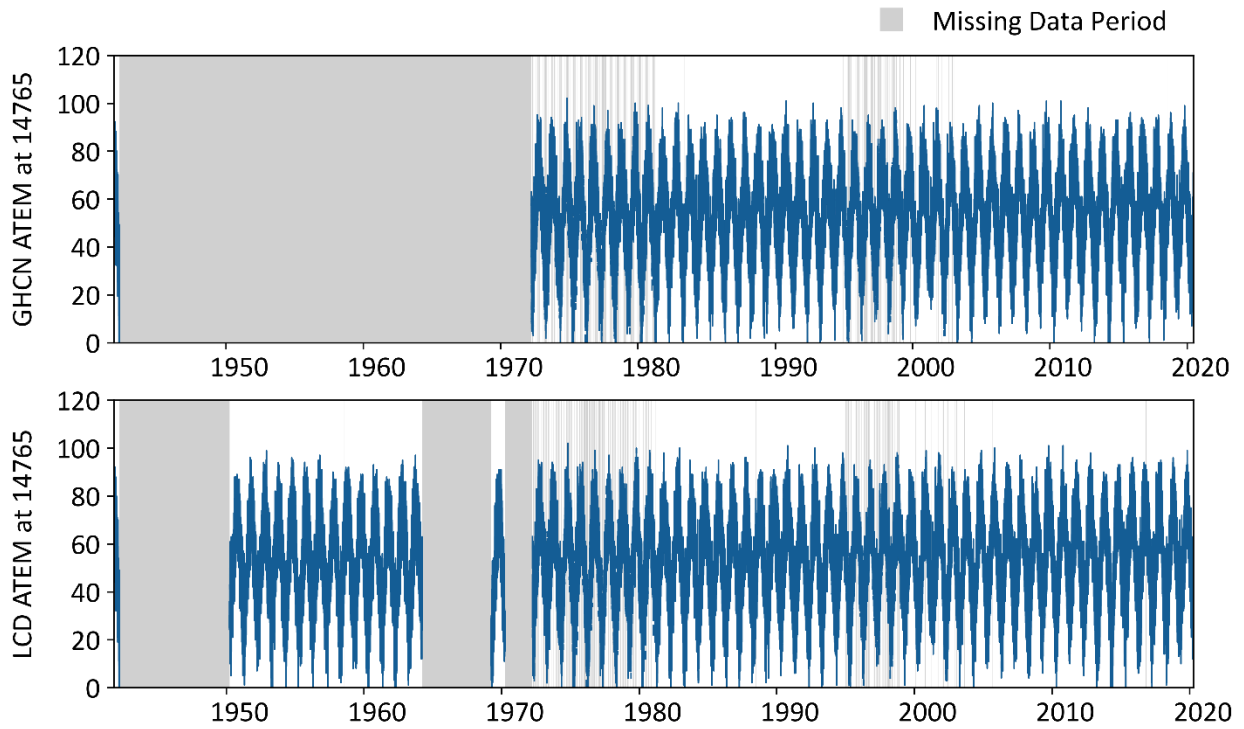
Figure A-11. The hourly temperature data at gage 72506814765.
