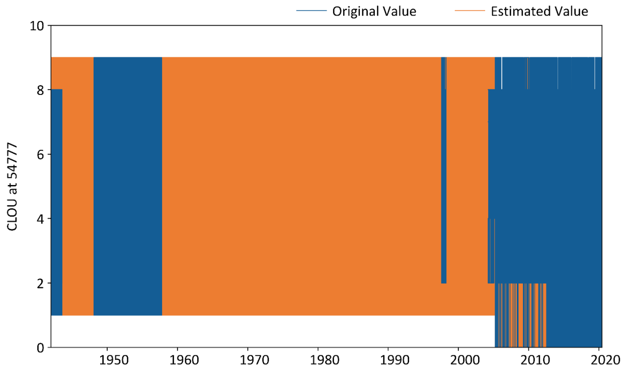
Figure A-25. The filled cloud cover data at gage 72506854777.
