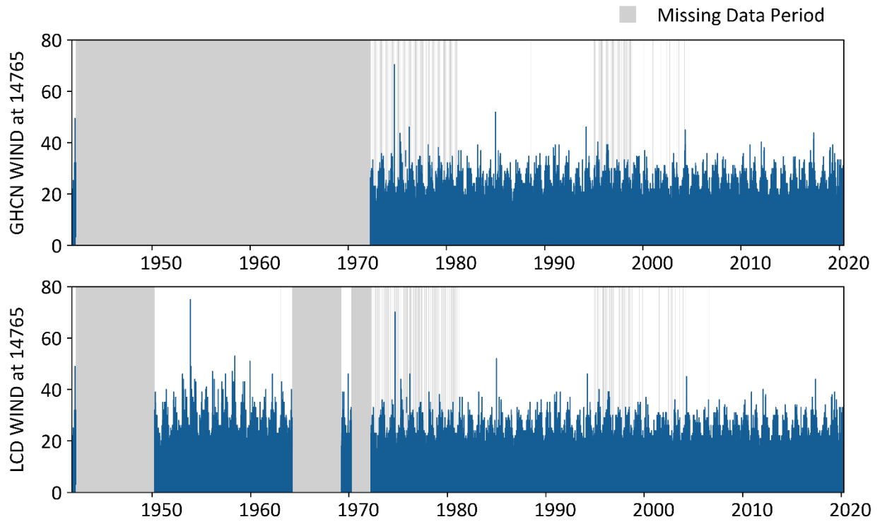
Figure A-1. The wind speed data at gage 72506814765.
