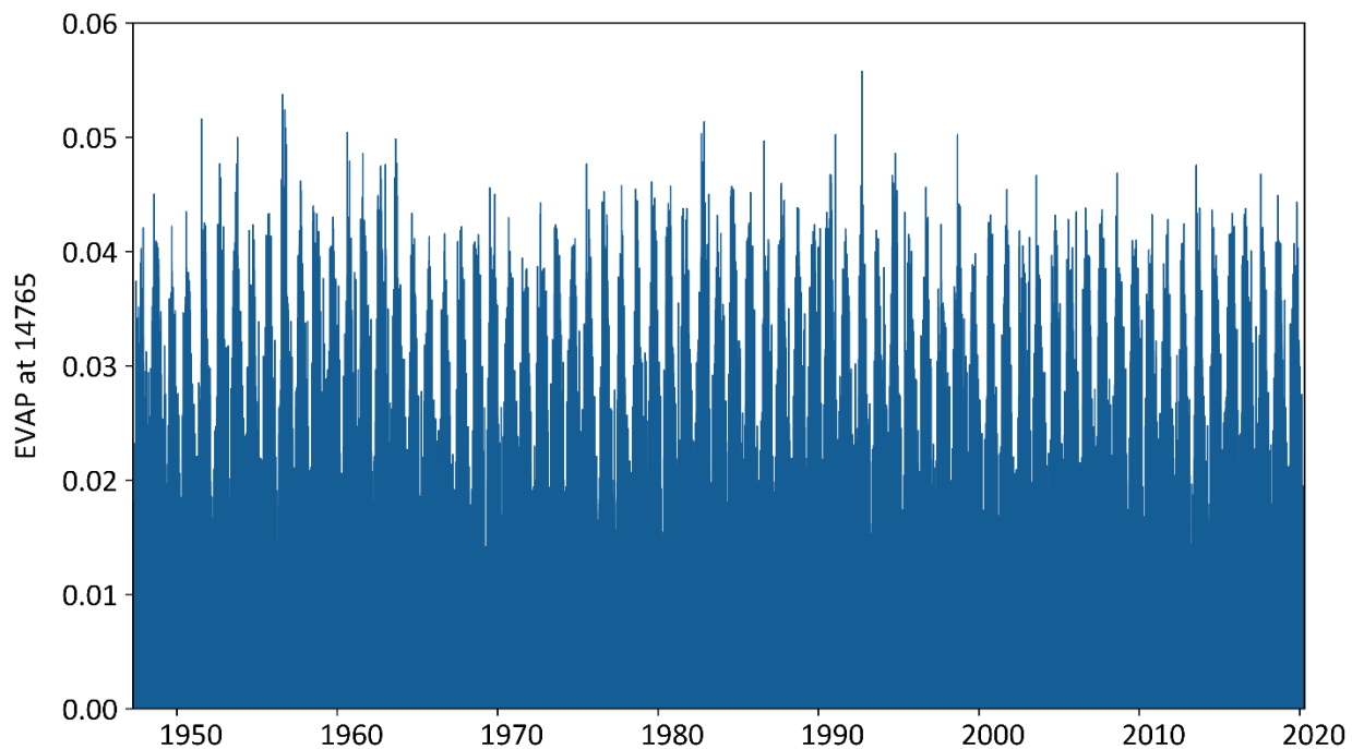
Figure A-28. The computed potential evapotranspiration data at gage 72506814765 using WDM Utility.
