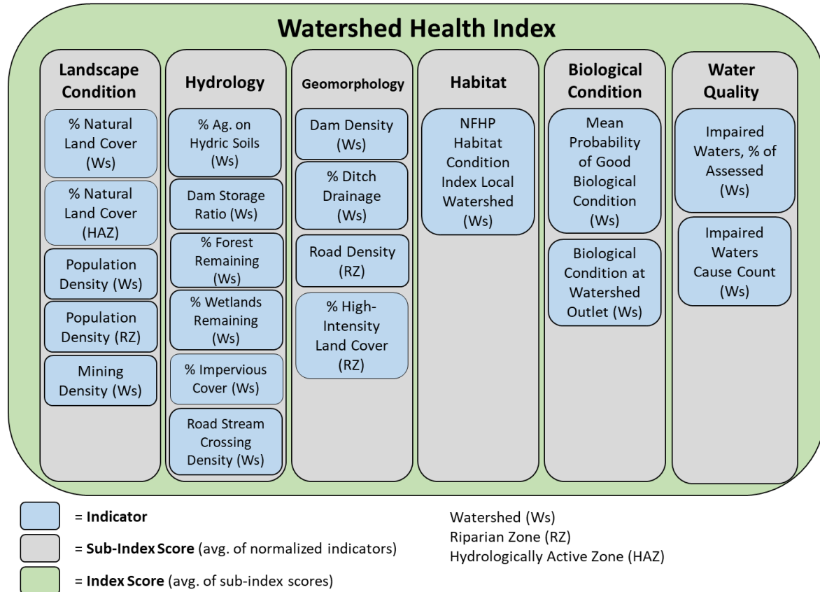
Figure 3. PHWA Watershed Health Index and Sub-Index structure with component indicators (blue boxes). Indicators measure watershed-wide (Ws), riparian zone (RZ) or hydrologically active zone (HAZ) attributes as marked.
