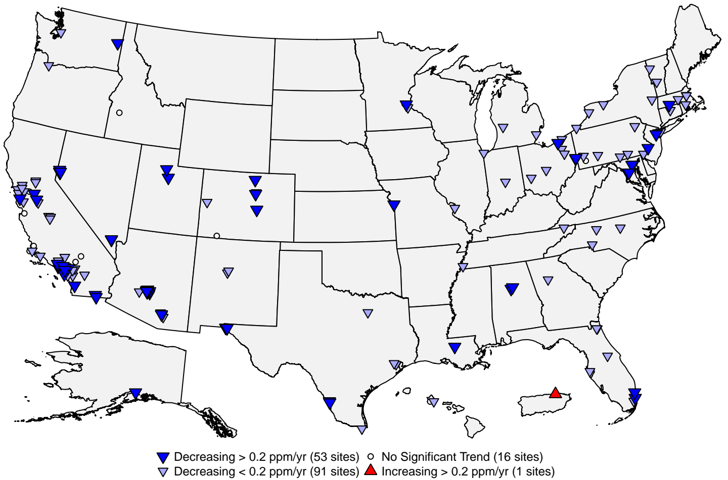
Figure 8: Site-level trends in 1-hour CO design values based on data from 2000 through 2021. Source: AQS, trends computed using R statistical software
