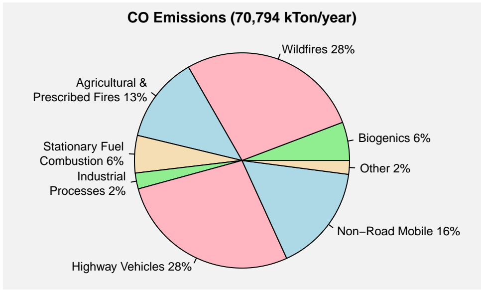
Figure 1. U.S. CO emissions by sector. Source: 2017 NEI .
