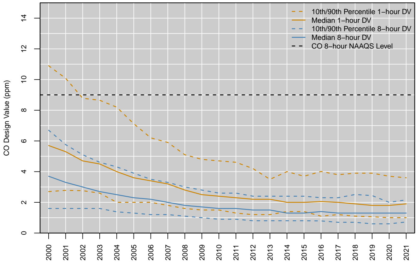
Figure 9: National trends in CO design values in ppm, 2000 to 2021. Source: AQS.
