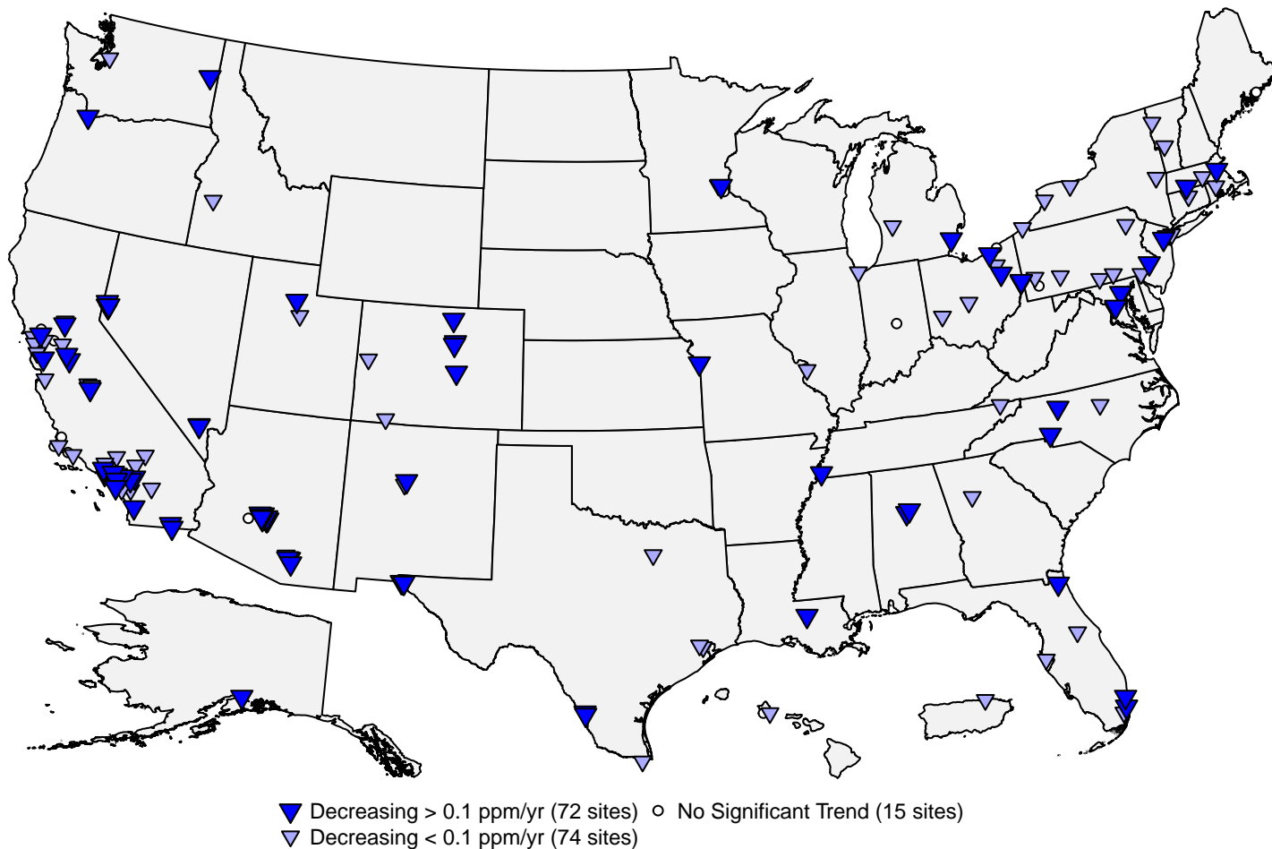
Figure 7: Site-level trends in 8-hour CO design values based on data from 2000 through 2021. Source: AQS, trends computed using R statistical software.
