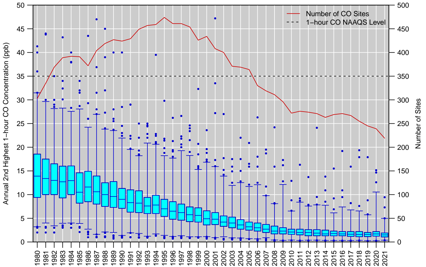
Figure 11: Distribution of annual 2nd highest 1-hour CO concentrations measured at U.S. monitoring sites, 1980 to 2021. Boxes represent the median and interquartile range, whiskers extend to the 1st and 99th percentiles, and values outside this range are shown as circles. The red line shows the number of CO monitoring sites reporting data to EPA in each year. Source: AQS.
