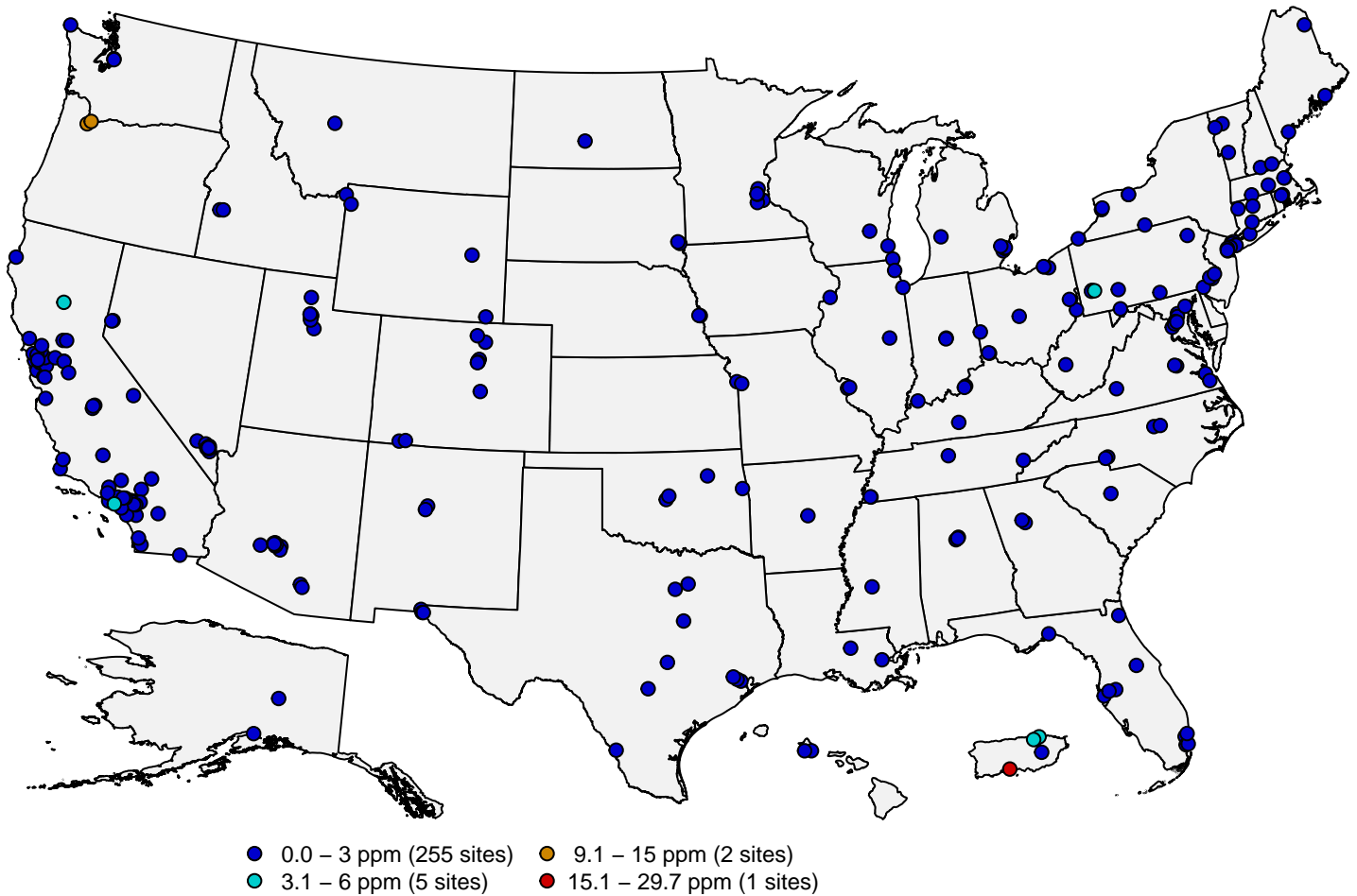
Figure 5: 8-hour CO design values in ppm for the 2020-2021 period. Source: AQS.
