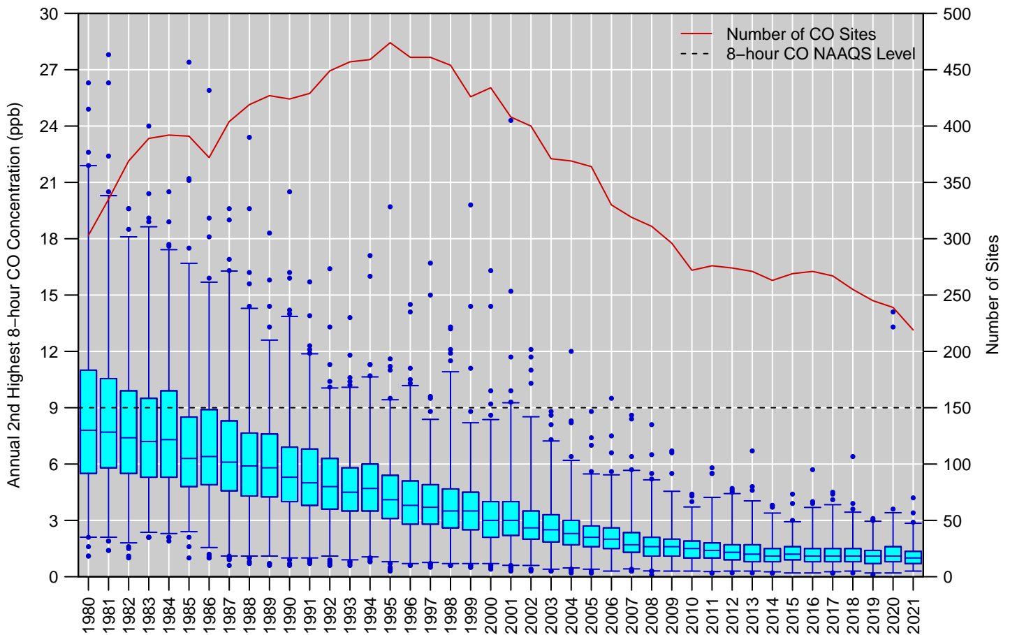
Figure 10: Distribution of annual 2nd highest 8-hour CO concentrations measured at U.S. monitoring sites, 1980 to 2021. Boxes represent the median and interquartile range, whiskers extend to the 1st and 99th percentiles, and values outside this range are shown as circles. The red line shows the number of CO monitoring sites reporting data to EPA in each year. Source: AQS.
