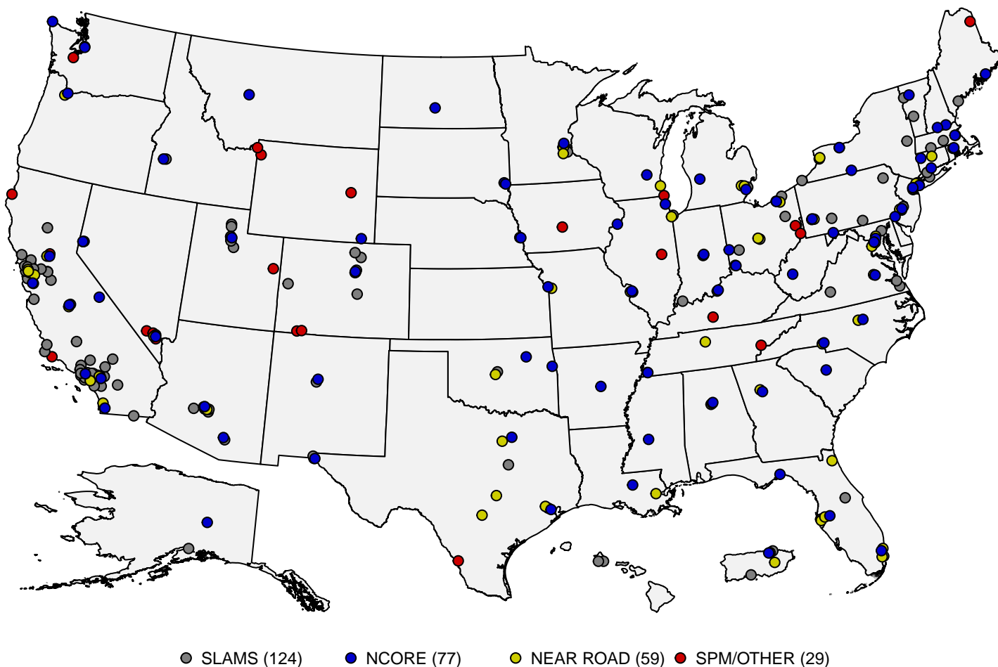
Figure 4: Map of U.S. CO monitoring sites reporting data to the EPA during the 2019-2021 period. Source: AQS .
