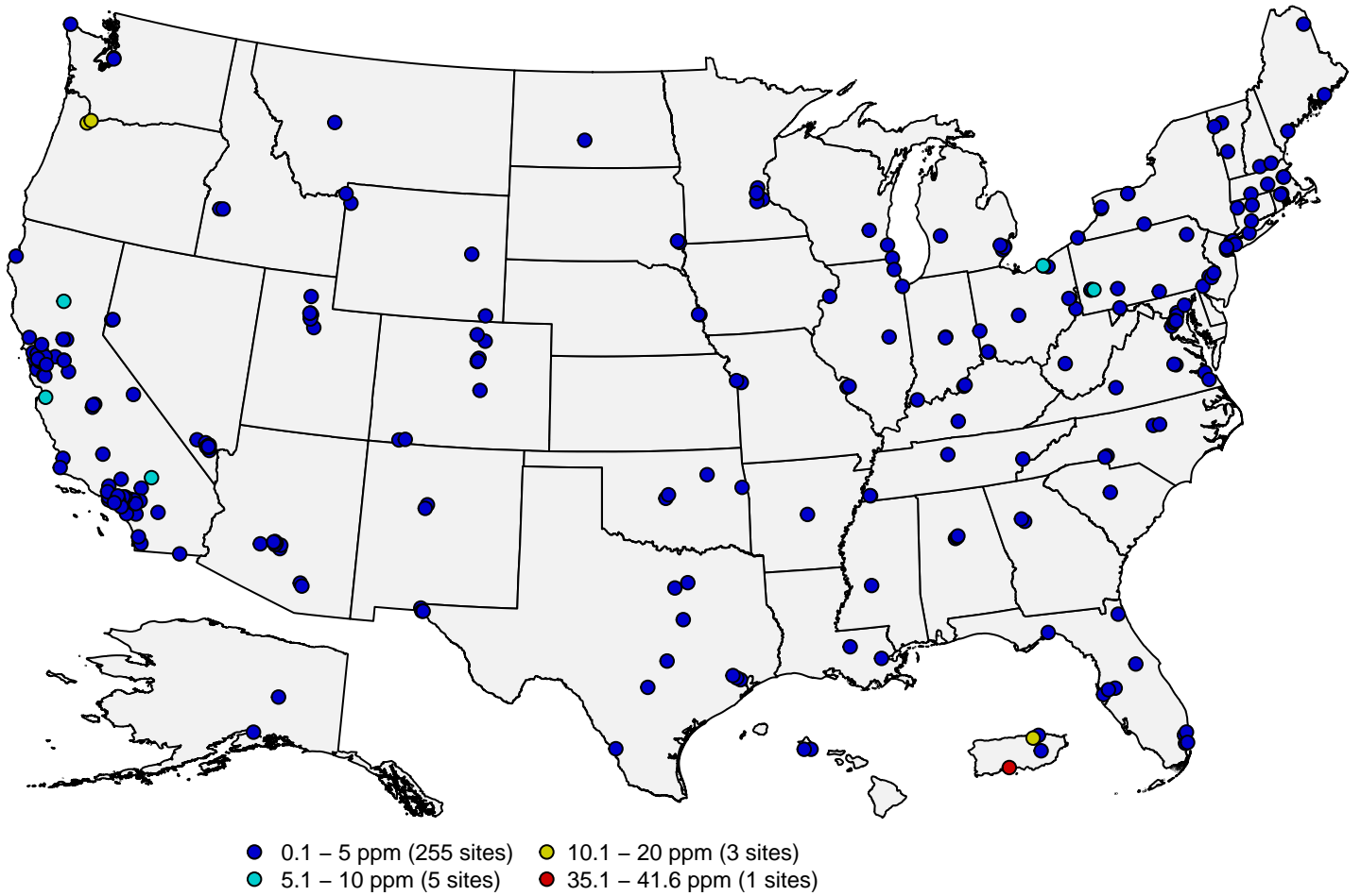
Figure 6: 1-hour CO design values in ppm for the 2020-2021 period. Source: AQS .
