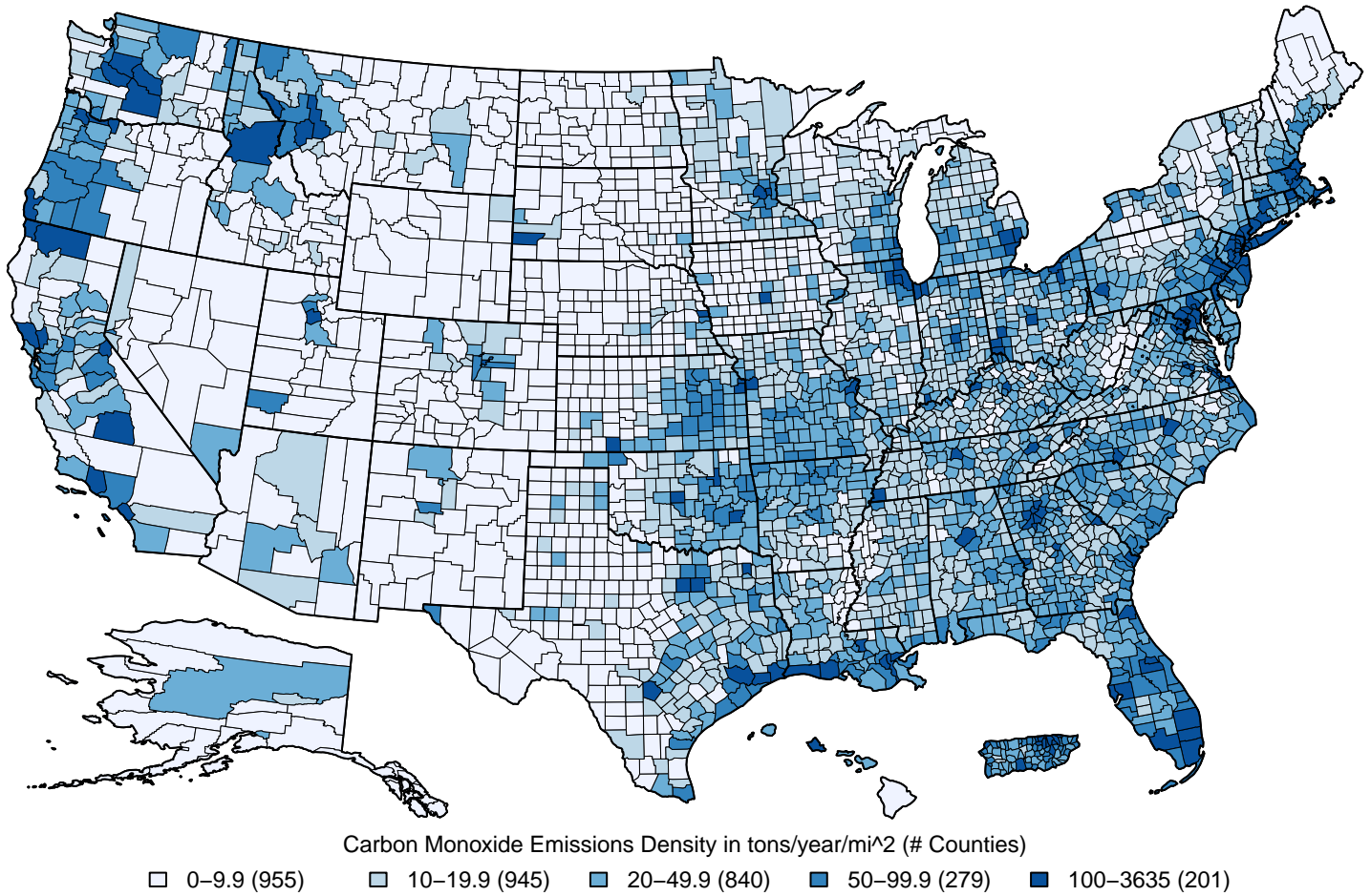
Figure 3. U.S. county-level CO emissions density estimates in tons/year/mi 2 . Source: 2017 NEI
