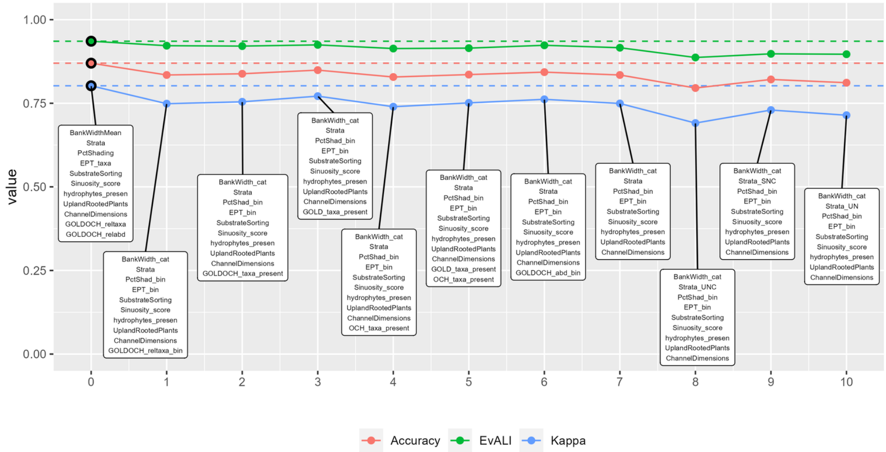
Figure 15. Impact of refinement of metric set on the model performance relative to the unstratified (no GIS) model using the training dataset. Each refinement description is relative the description at 0 (unstratified, no GIS model). Black circles indicate the highest Accuracy, EvALI, and Kappa scores. Dashed lines show performance of the unstratified (no GIS) model.
