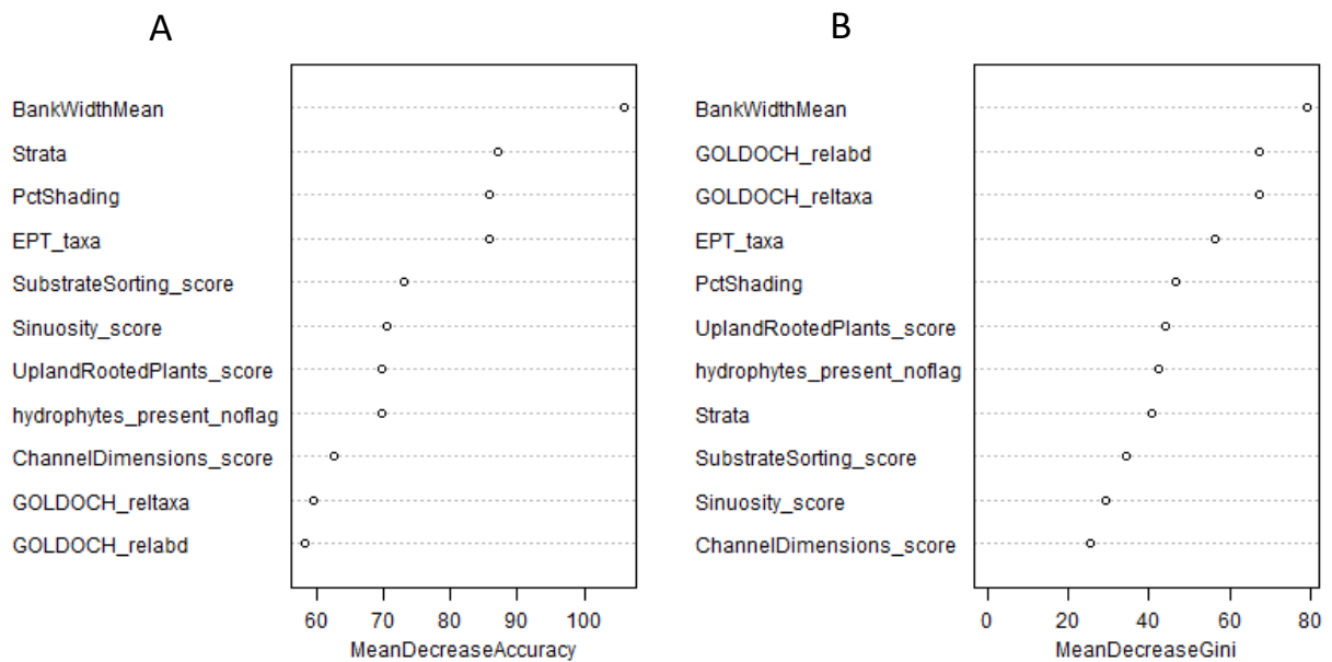
Figure 13: Metrics included in the unstratified (no GIS) model, by their order of importance. (A) Mean Decrease in Accuracy is the relative loss in predictive performance when the particular variable is omitted from the model. (B) Mean Decrease in Gini: Gini Index is a measure of node impurity, or how important the variable is in splitting between different streamflow duration classes.
