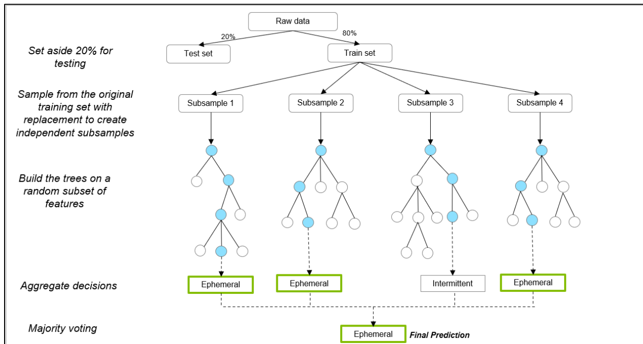
Figure 1. Random forest procedure used to determine a flow classification.
