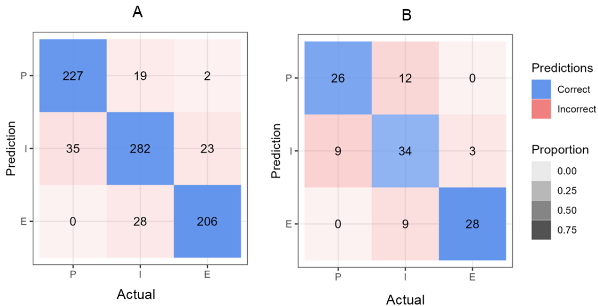
Figure 14. Confusion matrices of the (A) training vs (B) testing dataset on the unstratified (no GIS) model. The training dataset contained a total of 822 reach samples and the testing dataset contained 121 reach samples. X-axis shows actual flow duration class and Y-axis shows predicted flow duration class. Blue diagonal indicates correct predictions. P = perennial, I = intermittent, and E = ephemeral. Shading of boxes in matrices describe the proportion of reach samples in each dataset.
