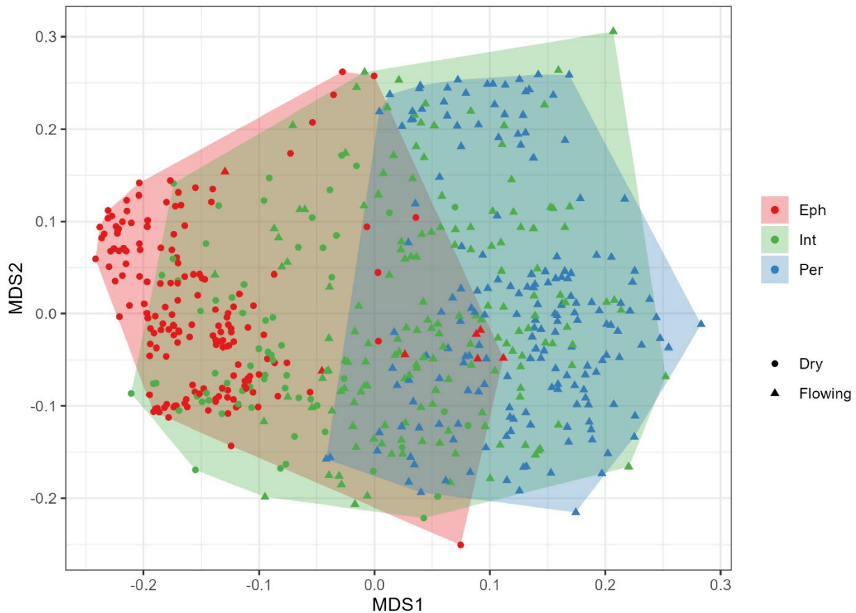
Figure 5. Beta SDAM GP candidate metric ordination.
