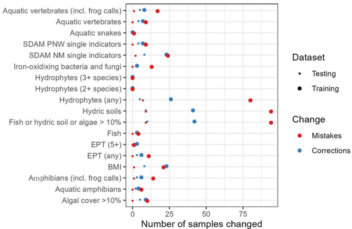
Figure 18. Influence of single indicators on performance of the refined model
