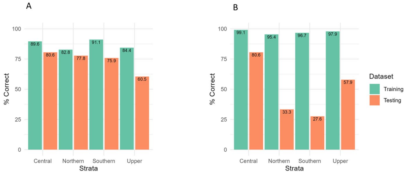
Figure 11: Accuracy of the (A) unstratified GP model without GIS metrics and (B) unstratified GP model with GIS metrics based on training and testing datasets by strata (943 total observations). Numbers shown in bars are the percent of correctly classified samples as perennial, intermittent, or ephemeral.
