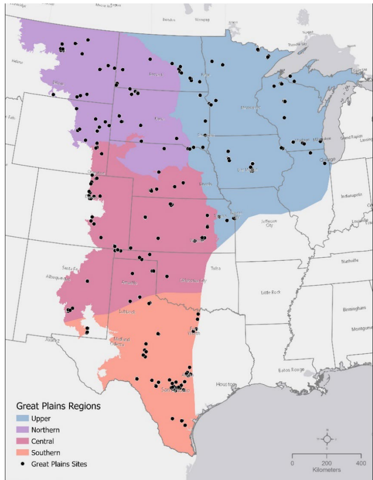
Figure 3: The four GP sub-strata; study reaches shown are those used to calibrate the beta SDAM GP.
