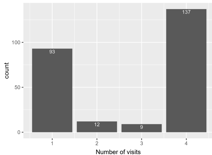
Figure 6. Distribution of number of visits across the 251 study reaches. Numbers inside of bars are the number of study sites with 1, 2, 3 or 4 visits.
