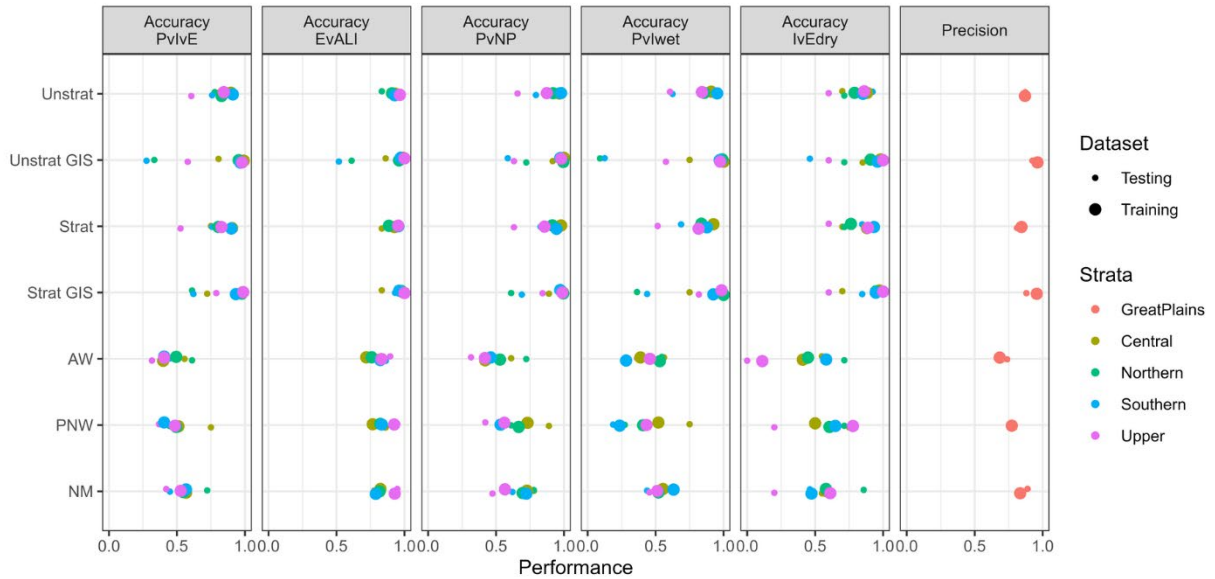
Figure 10. Performance of the various model sets evaluated within strata defined by sub-region. PvlvE: Proportion of reach samples classified correctly as perennial, intermittent, or ephemeral. The y-axis labels on the left indicate the stratifications used to develop the models (if any). EvAlI: Proportion of reach samples classified correctly as ephemeral or at least intermittent. PvNP: Proportion of reach samples classified correctly as perennial or non-perennial. Pvlwet: Proportion of flowing classified correctly as perennial or intermittent. IvEdry: Proportion of dry reach samples correctly classified as intermittent or ephemeral. Model sets are described in Table 5. AW: Results for the Beta SDAM AW; PNW: Results for the SDAM PNW; NM: Results for the SDAM NM.
