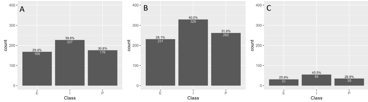
Figure 8: Distribution of ephemeral (E), intermittent (I), and perennial (P) classes in the (A) training dataset before oversampling, (B) training dataset after oversampling, and the (C) testing dataset. Shown for each bar is the number of samples for a streamflow duration class and the percent of samples within the datasets. A balanced distribution between classes is important to mitigate against bias and improve model accuracy.
