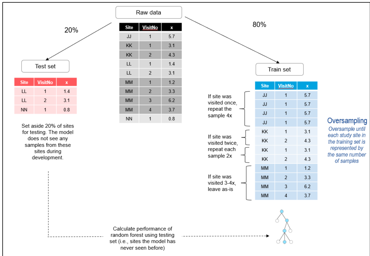
Figure 7. Oversampling process used for training dataset. x is a hypothetical candidate indicator
