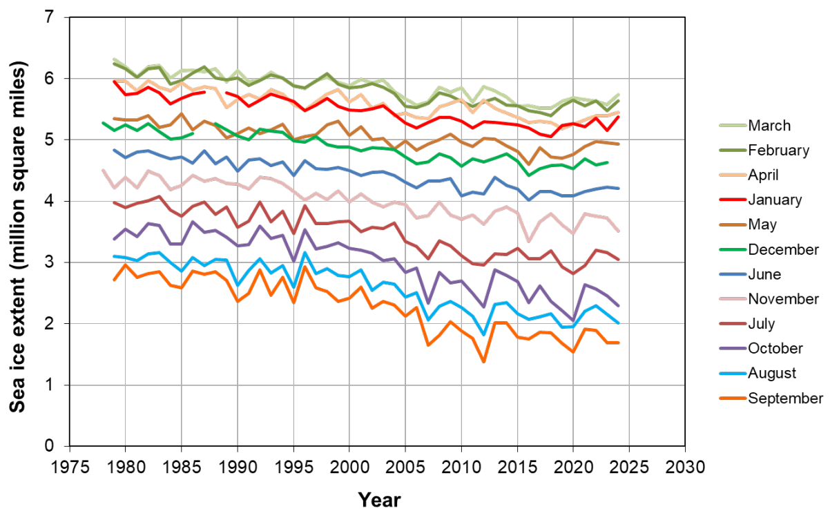
Figure TD-1. Arctic Sea Ice Extent for Each Month, 1978/1979–2023/2024
