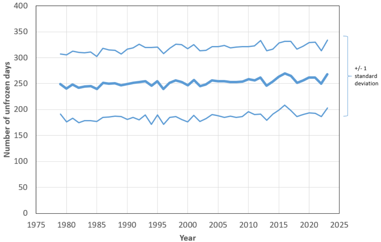
Figure TD-3. Number of Unfrozen Days in the Contiguous 48 States and Alaska, 1979–2023, with Standard Deviation Showing Geographic Variation
