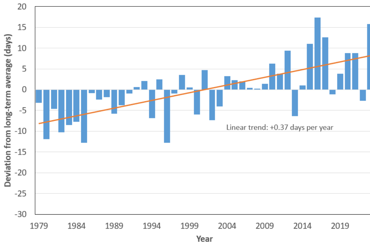
Figure TD-2. Number of Unfrozen Days in the Contiguous 48 States and Alaska, 1979–2023
