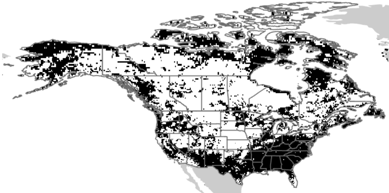
Figure TD-4. Significance of 1979–2023 Trends in the Annual Number of Unfrozen Days
